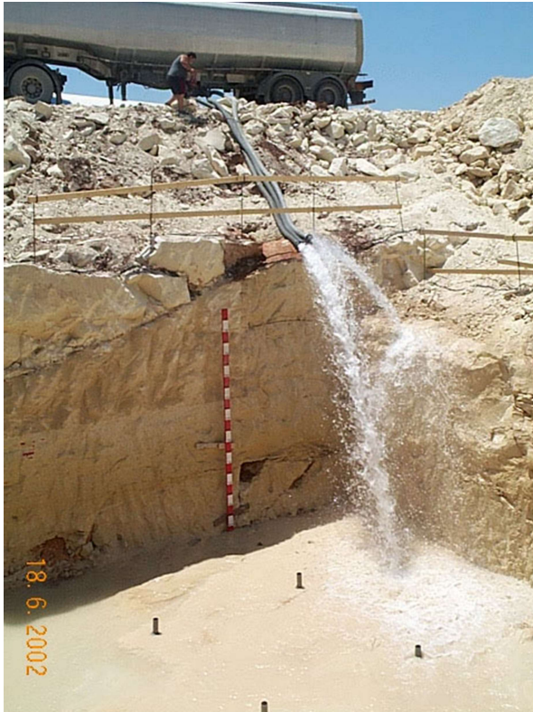
Figure 60: MDH soakaway under test
