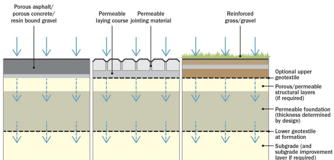
Figure 77: Pervious pavement cross section showing various types
